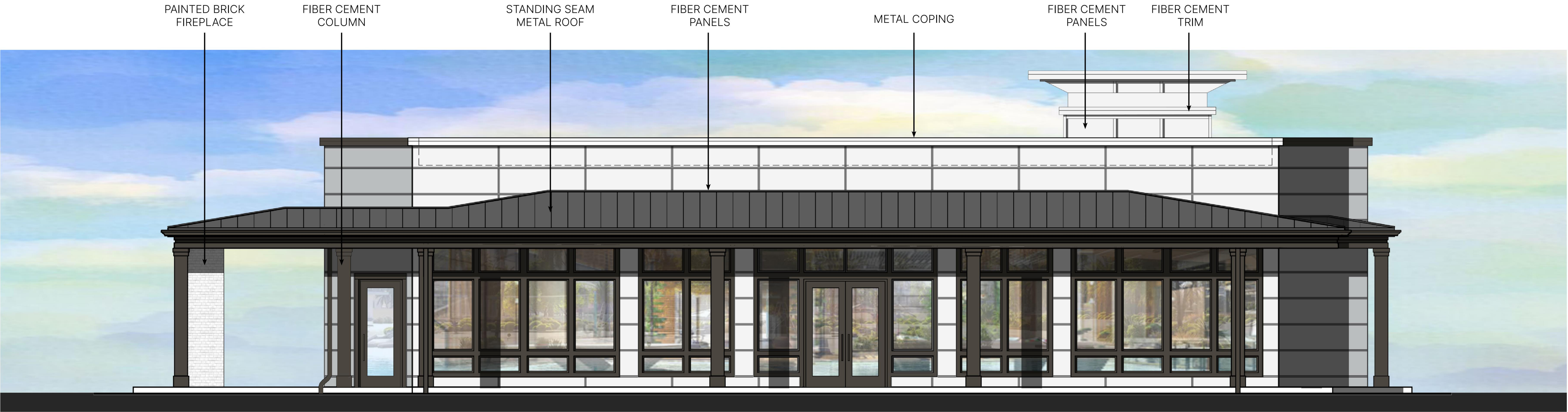
CLUBHOUSE NORTH ELEVATION
